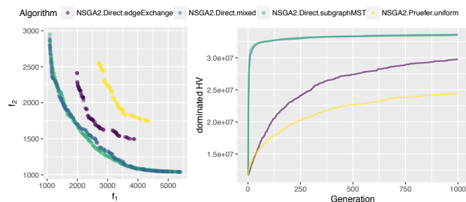
Fig. 8. Left: exemplary approximations of the Pareto-front for all considered combinations of tree encodings and mutation operators. Right: the optimization trace of the dominated hypervolume resulting in the corresponding approximations in the left plot. Clearly, the sub-tree mutation with/without intermingled edge exchange advances to the Pareto-front rapidly, while the other mutations exhibit inferior performance.
